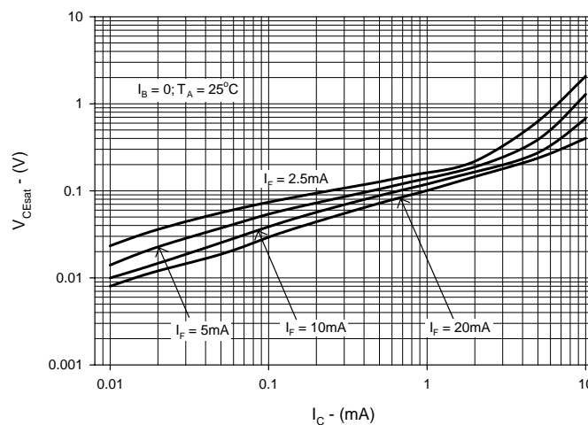
Fig. 11 Collector-Emitter Saturation Voltage as a Function of Collector Current
