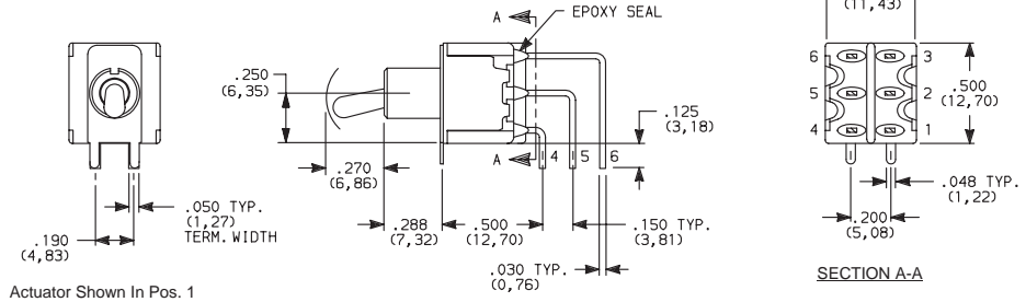
7201MD9AV2BE Vertical Actuation DPDT
