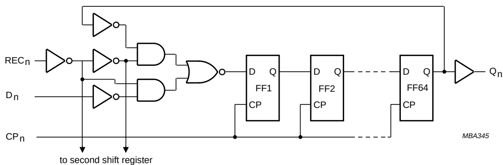
Fig.3 Logic diagram.
