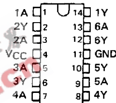
SN5404 . . . W PACKAGE (TOP VIEW)
