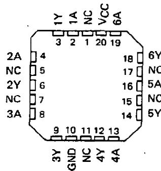
SN54LS04, SN54S04 . . . FK PACKAGE (TOP VIEW)
