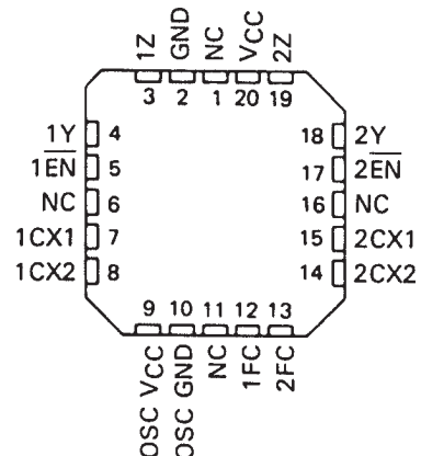
SN54LS626 . . . FK PACKAGE
