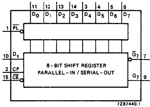
Fig.4 Functional diagram.
