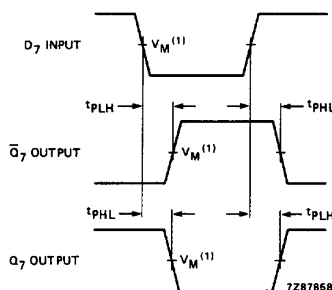
Fig.8 Waveforms showing the data input ( D_n ) to output ( Q_7 or \bar{Q}_7 ) propagation delays when \bar{PL} is LOW.
