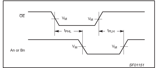
Waveform 4. Propagation Delay for \overline{OE} to An or Bn Outputs (74F641) (Bn or An Inputs in Low State)
