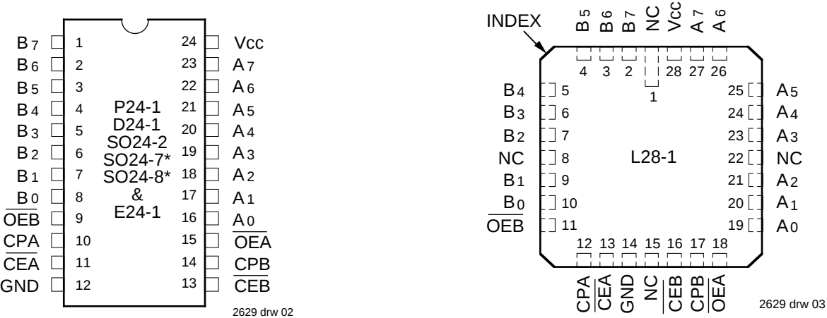
DIP/SOIC/SSOP/QSOP/CERPACK TOP VIEW * For 29FCT52/29FCT2052AT/BT/CT only
