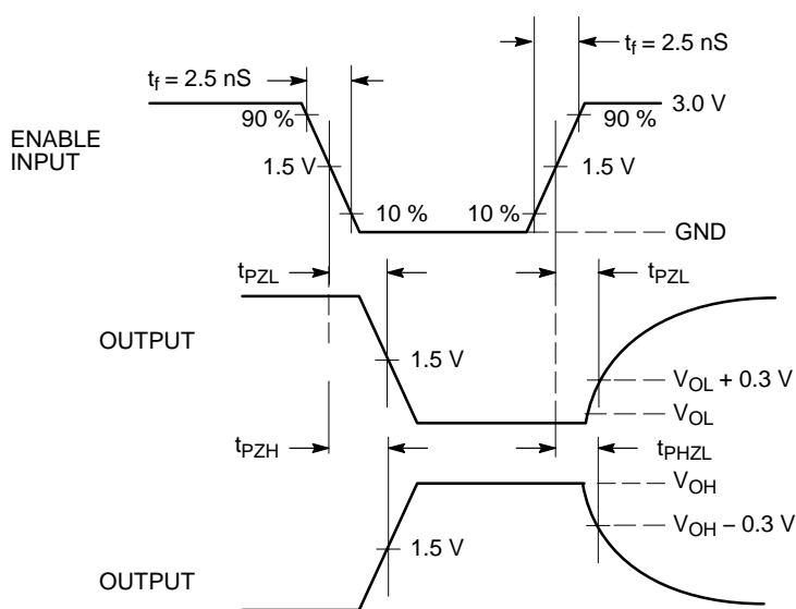
Figure 5. Enable/Disable Delays
