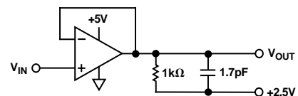
Circuit Diagram
