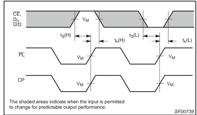
Waveform 6. Data Set Up and Hold Times
