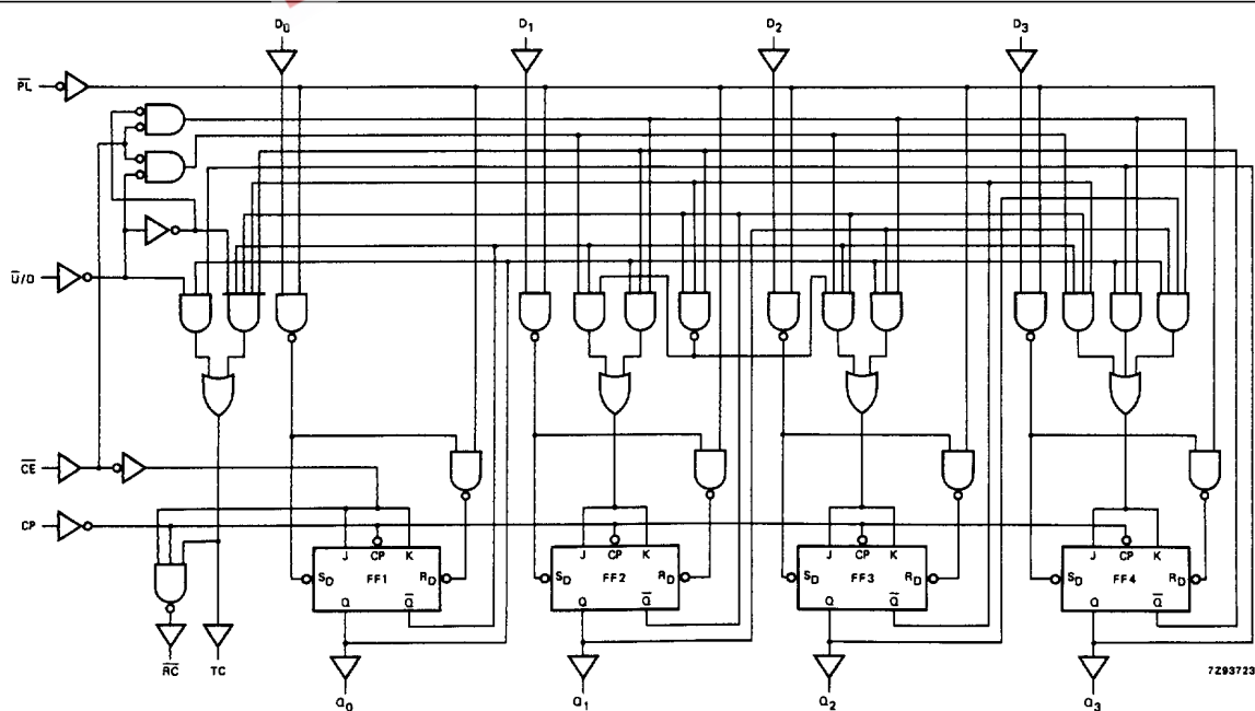
Fig.9 Logic diagram.
