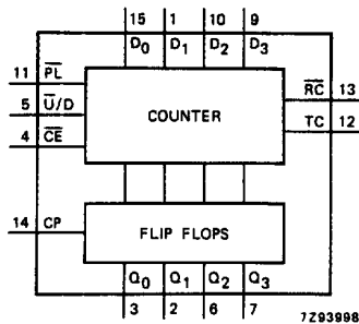
Fig.4 Functional diagram.
