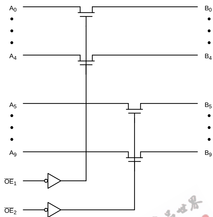
Figure 2. Logic Diagram
