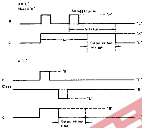
Fig.1 Typical Input/Output Pulses
