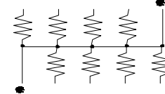
745X102 8 Resistors 10 Terminations
