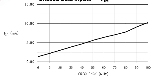
Typical I_{CC} vs Output Switching Frequency C_L = 0\text{ pF} , V_{CC} = V_{IH} = 5.5\text{V} , LE = GND, 1 Output Switching at 50% Duty Cycle Data to Output, Transparent Mode with Unused Data Inputs = V_{IH}
