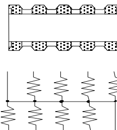
746X101 8 Resistors 10 Terminations
