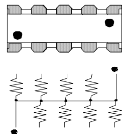
745X102 8 Resistors 10 Terminations
