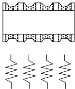
742C083 4 Resistors 8 Terminations
