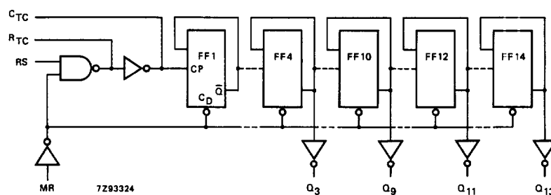
Fig.5 Logic diagram.
