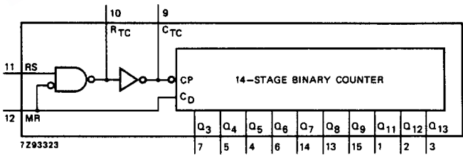
Fig.4 Functional diagram.
