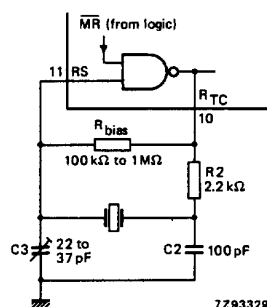
Fig.11 External components connection for a crystal oscillator.
