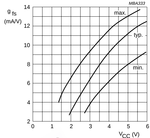
Fig.8 Typical forward transconductance g_{fs} as a function of the supply voltage V_{CC} at T_{amb} = 25\text{ °C} .
