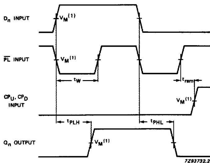
Fig.9 Waveforms showing the parallel load input ( \overline{\text{PL}} ) and data (D n ) to Q n output propagation delays and \overline{\text{PL}} removal time to clock input (CP U , CP D ).
