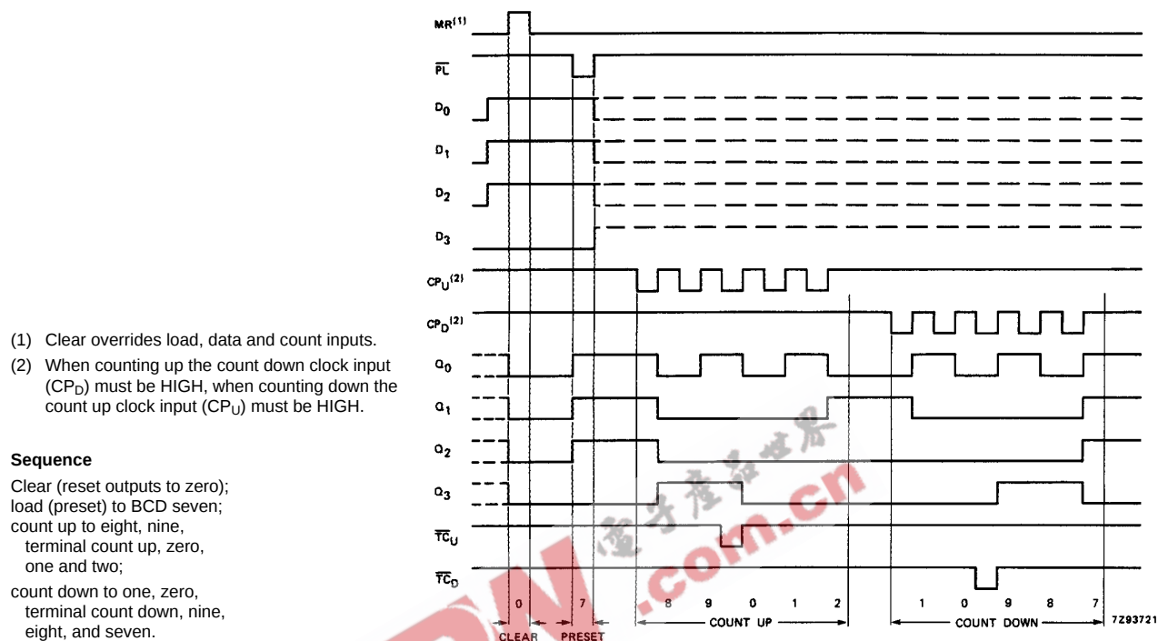
Fig.5 Typical clear, load and count sequence.
