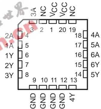
54ACT11034 . . . FK PACKAGE (TOP VIEW)
