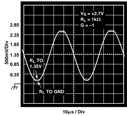
Figure 35. Output Swing
