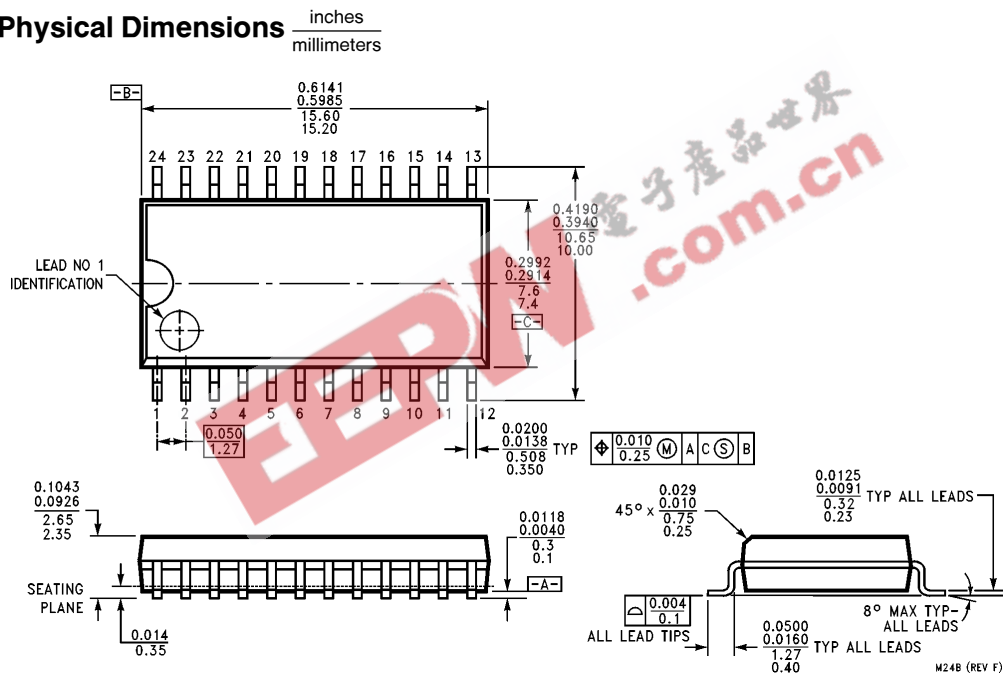
24-Lead (0.300" Wide) Small Outline Package Order Number 74LVX3L383WM or 74LVX3L383WMX NS Package Number M24B
