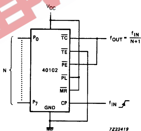
Fig.14 Divide-by-N counter.
