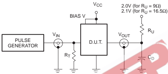
Test Circuit for Outputs on B Port
