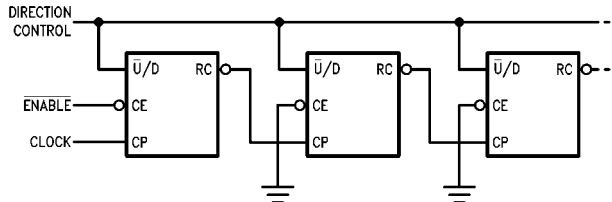
FIGURE 1. N-Stage Counter Using Ripple Clock
