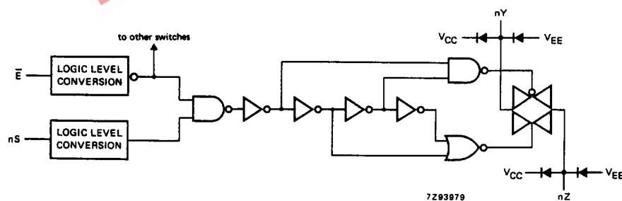
Fig.5 Schematic diagram (one switch).
