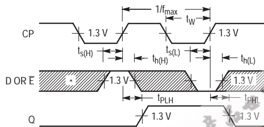
AC WAVEFORM
