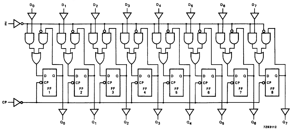
Fig.5 Logic diagram.
