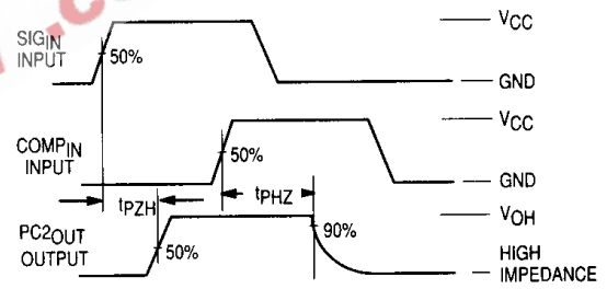
Figure 2. Switching Waveforms
