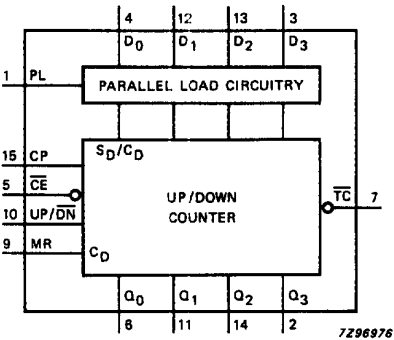
Fig.4 Functional diagram.
