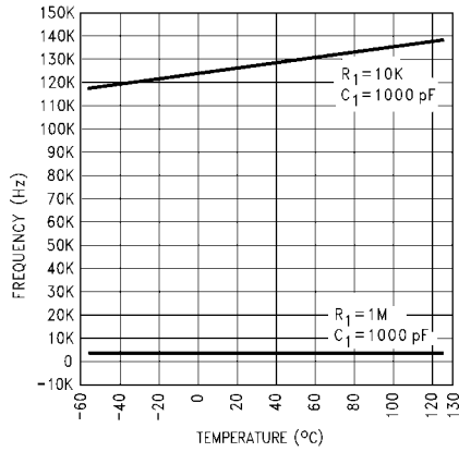
VHC4046 VCO out vs Temperature V CC = 4.5V R 2 =OPEN VCO N =V CC /2
