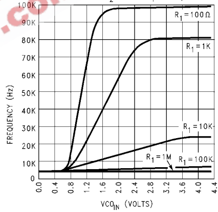
VHC4046 VCO IN vs f OUT V CC = 4.5V
