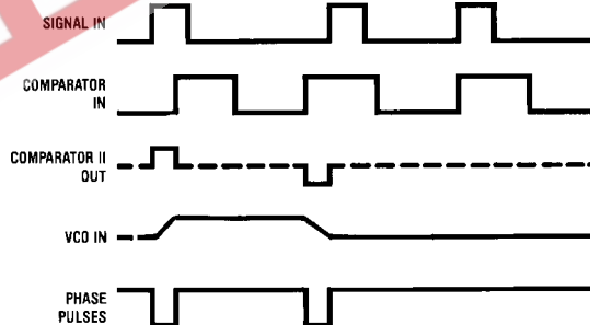
FIGURE 6. Typical Phase Comparator II Output Waveforms
