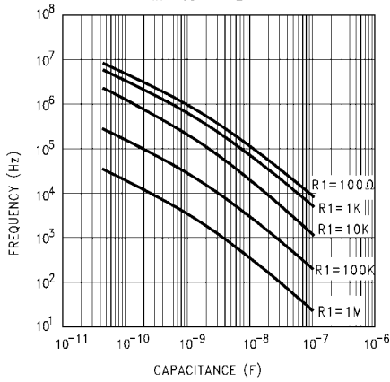
Typical Center Frequency vs R_1, C_1 V_{CC} = 4.5V V_{CO,N} = V_{CC}/2 R_2 = OPEN
