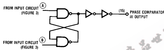
FIGURE 7. Phase Comparator III Logic Diagram
