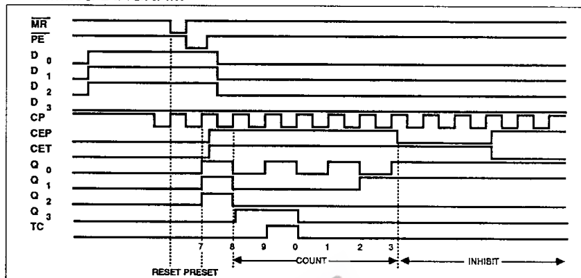
TIMING DIAGRAM
