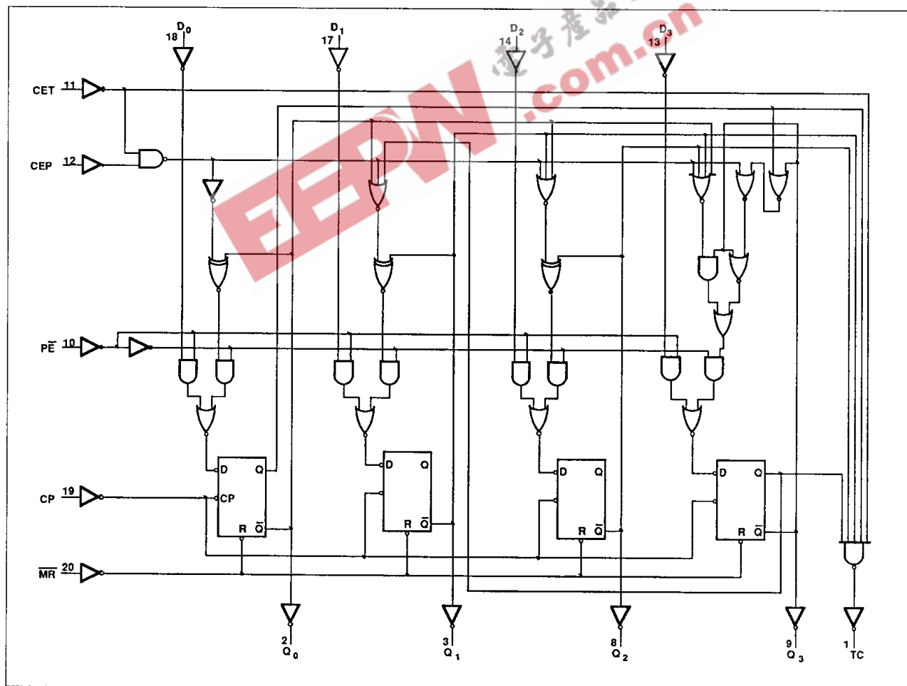
LOGIC DIAGRAM
