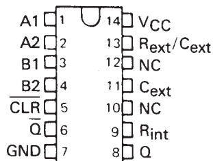
SN54122, SN54LS122 . . . J OR W PACKAGE SN74122 . . . N PACKAGE SN74LS122 . . . D OR N PACKAGE (TOP VIEW) (SEE NOTES 1 THRU 4)
