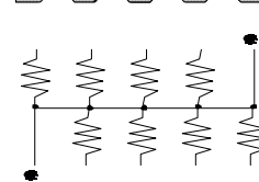
745X102 8 Resistors 10 Terminations
