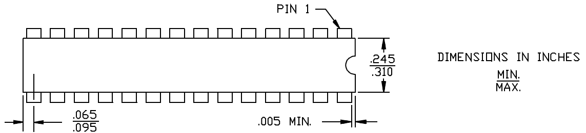
28-pin (300-Mil) CerDIP D22 MIL-STD-1835 D-15 Config. A
