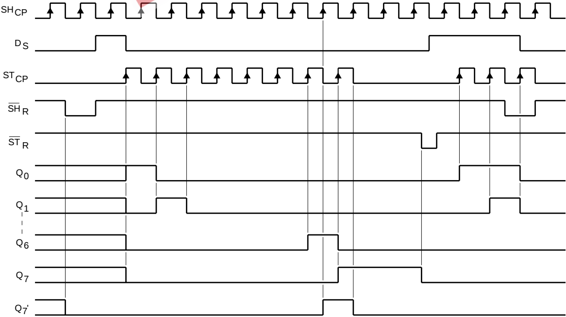
Fig.6 Timing diagram.
