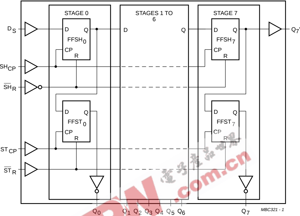
Fig.5 Logic diagram.
