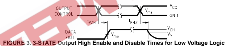
FIGURE 3. 3-STATE Output High Enable and Disable Times for Low Voltage Logic
