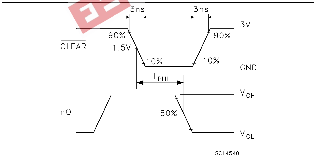
Figure 5: Waveform - Propagation Delays ( f=1\text{MHz} ; 50% duty cycle)
