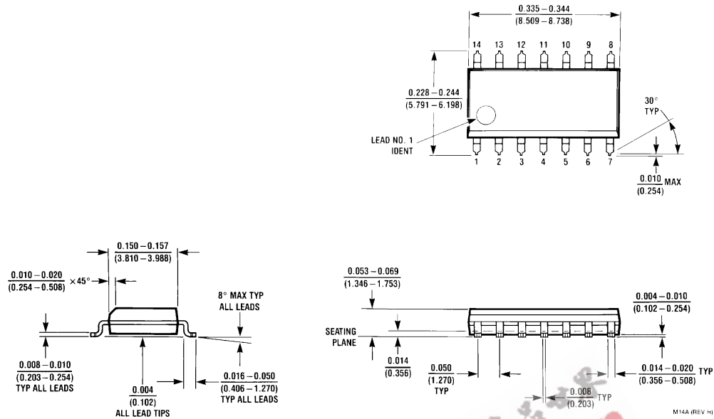
14-Lead Small Outline Integrated Circuit—JEDEC (M) NS Package Number M14A
