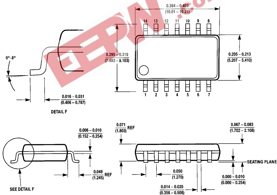
14-Lead Small Outline Package—EIAJ (SJ) NS Package Number M14D
