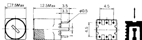
(Unit: mm)
