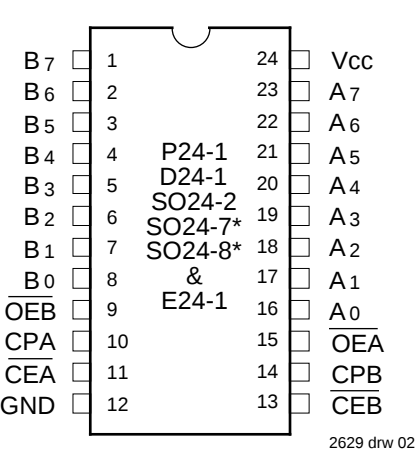
DIP/SOIC/SSOP/QSOP/CERPACK TOP VIEW
