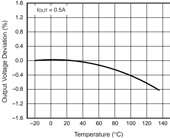
Fig. 5 – Temperature Stability
