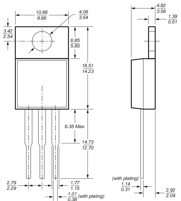
TO-220
