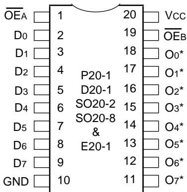
DIP/SOIC/QSOP/CERPACK TOP VIEW
