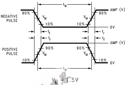
FIGURE 2a. Test Input Signal Levels
