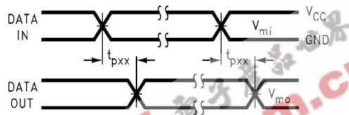
FIGURE 2. Waveform for Inverting and Non-Inverting Functions
