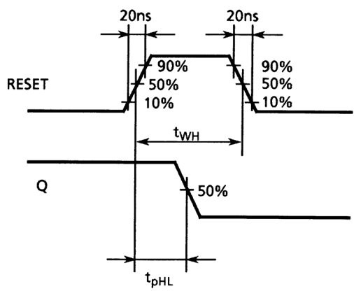
Waveform 2
