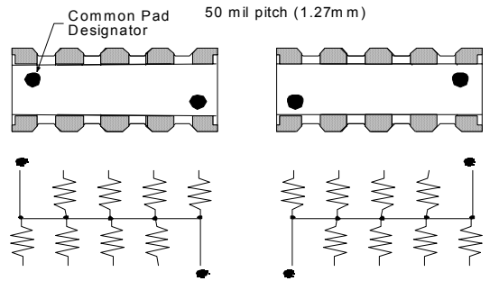
745X101 8 Resistors 10 Terminations 745X102 8 Resistors 10 Terminations
