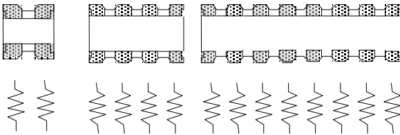
741X043 2 Resistors 4 Terminations 741X083 4 Resistors 8 Terminations 741X163 8 Resistors 16 Terminations
