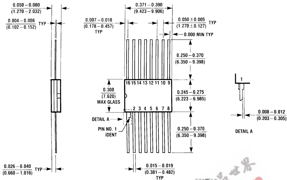
16-Lead Ceramic Flat Package (W) Order Number 54153FMBQ or DM54153W NS Package Number W16A
