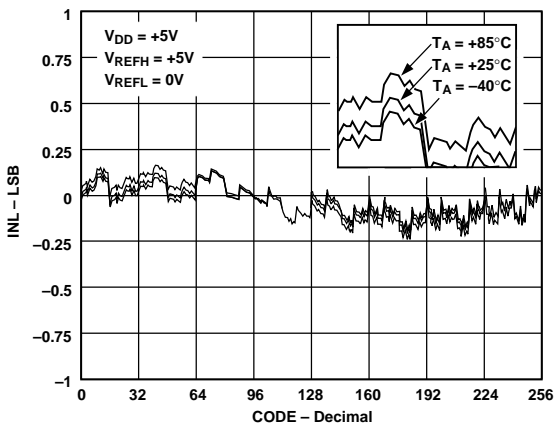
Figure 7. INL vs. Code
