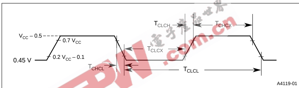
Figure 16. External Clock Drive Waveforms
