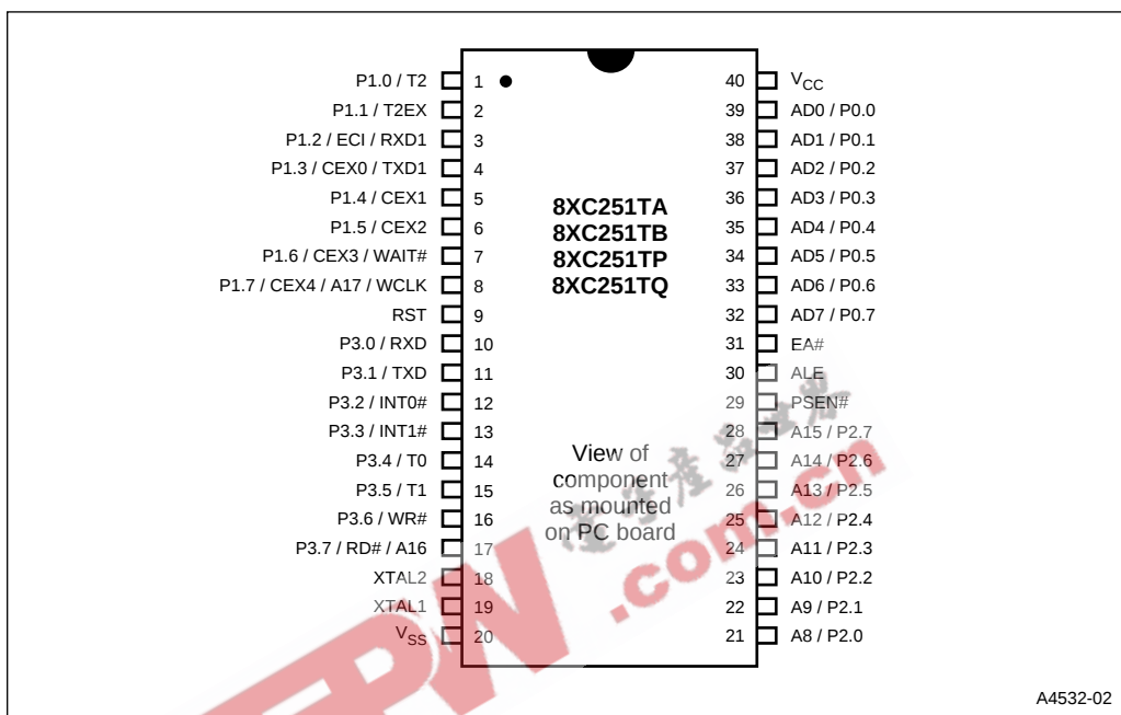
Figure 4. 8xC251TA/TB/TP/TQ 40-pin PDIP Packages
