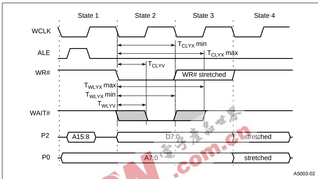
Figure 14. External Bus Cycle: Data Write (Page Mode)
