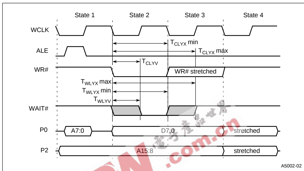
Figure 12. External Bus Cycle: Data Write (Nonpage Mode)
